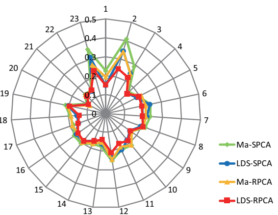
Fig. 2. RMSEs of different feature dimension reduction algorithms and different smoothing methods for on-line vigilance estimation
