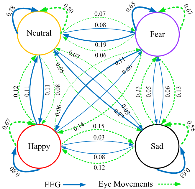
Fig. 11. Confusion graph of EEG and eye movements, which shows their complementary characteristics for emotion recognition. [The numbers denote the percentage values of samples in the class (arrow tail) classified as the class (arrow head). Bolder lines indicate higher values.]
