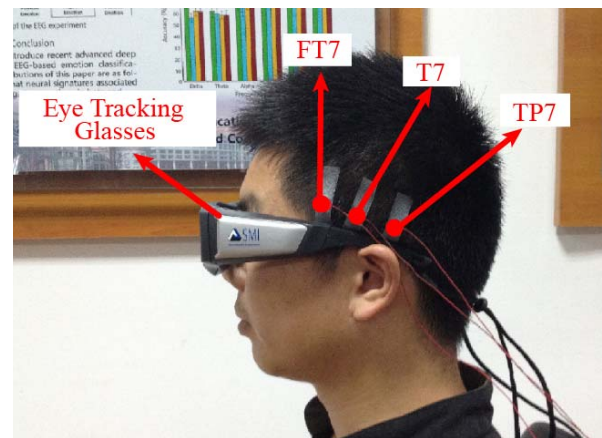
Fig. 5. Setup for the EmotionMeter hardware. The six symmetrical temporal electrodes above the ears are used for EEG recordings. The eye movement parameters are extracted from the wearable eye-tracking glasses.
