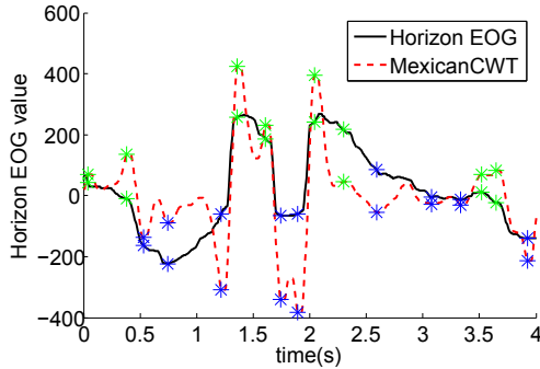
Fig. 4. The saccade detection segment
