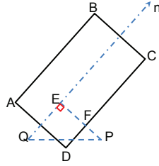
Figure 7: Definition of cylindricity error.
