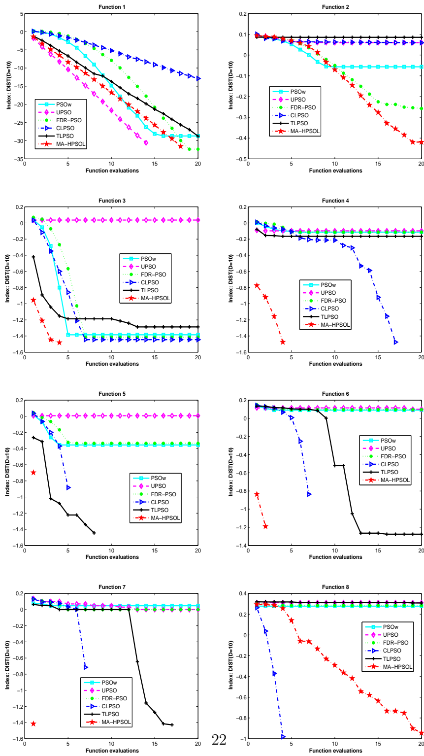
Figure 6: The median \text{dist}(D) values of 10-D test functions.
