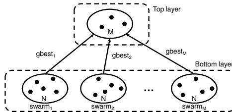
Figure 1: The architecture of two-layer hierarchical PSO.
