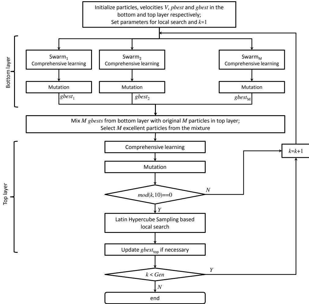
Figure 3: Flow chat of proposed algorithm (MA-HPSOL).
