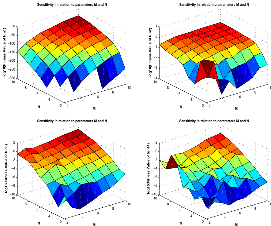
Figure 4: MA-HPSOL sensitivity in relation to M and N .
