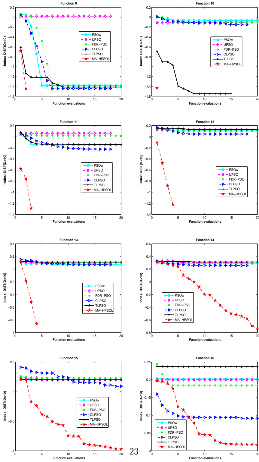
Figure 6: (continued) The median dist(D) values of 10-D test functions.
