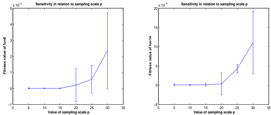
Figure 5: MA-HPSOL sensitivity in relation to sampling scale p .
