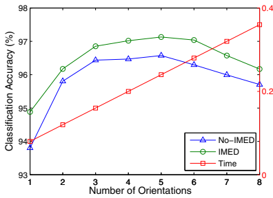
Fig. 4. The average accuracy over all 10 datasets using different orientation numbers and with/without IMED transform. The approximate computing time is also given.
