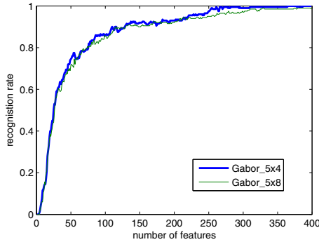
Fig. 3. Face recognition performance of the PCA method with two different sets of Gabor filters: Gabor 5 × 4 and Gabor 5 × 8
