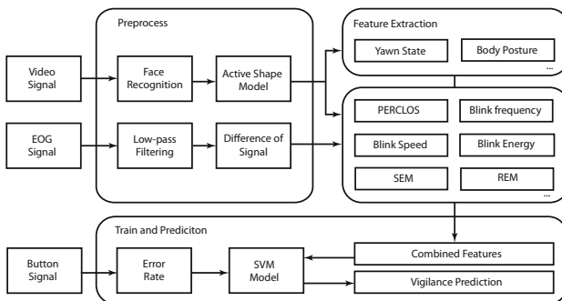
Fig. 1. The proposed vigilance analysis system by combining video and EOG features
