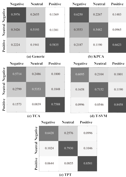
Figure 5: The confusion matrices of the five methods.
