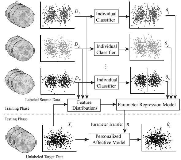
Figure 2: The framework of the transductive parameter transfer (TPT) approach adopted in this work.
